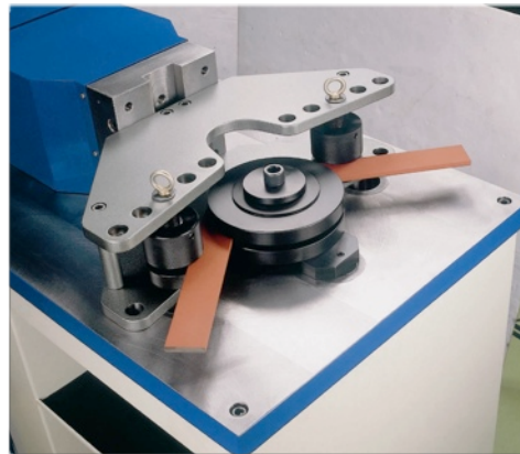
Flat Bar Bending Tool
