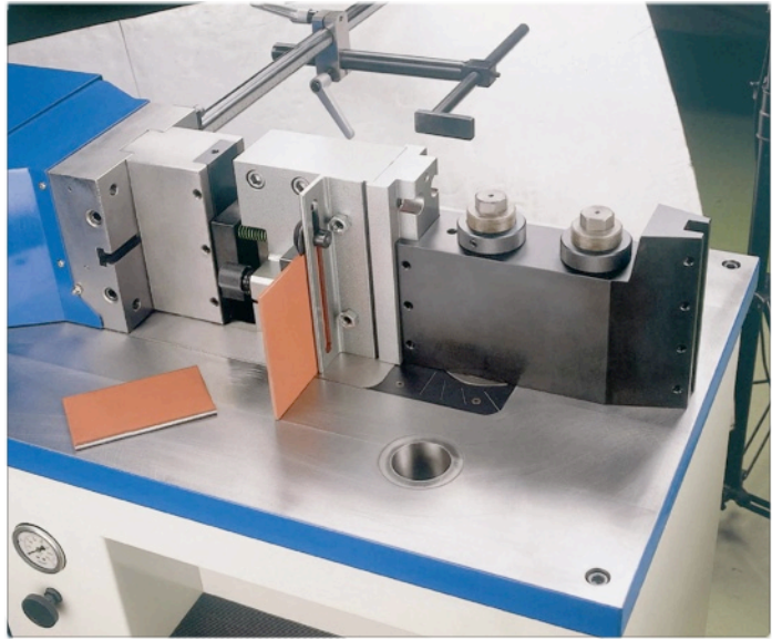
Flat Bar Shearing Tool
