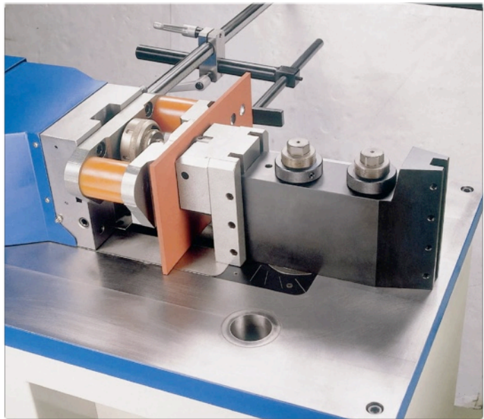
Punching Tool
